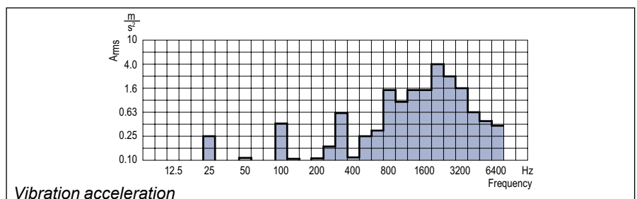
Vibration acceleration
