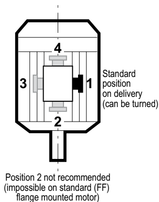
Positions of the threaded plug in relation to the drive end
