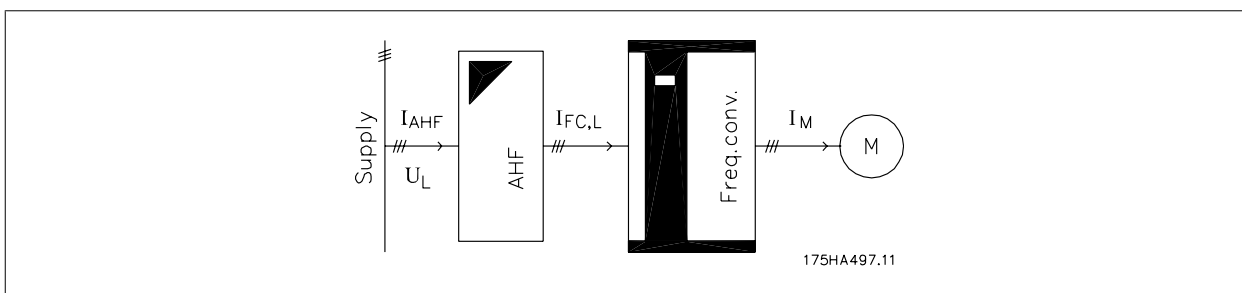
Illustration 2.1: Principle connection diagram of the Danfoss harmonic filter.
