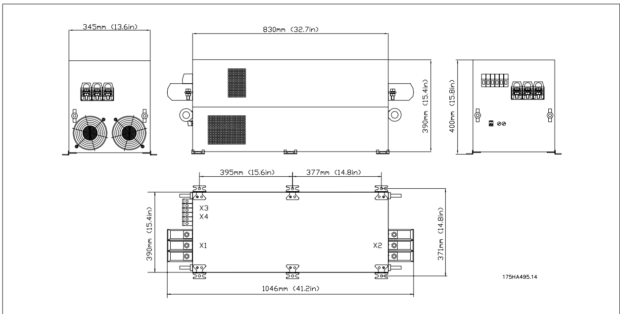
Illustration 3.4: Frame size E
