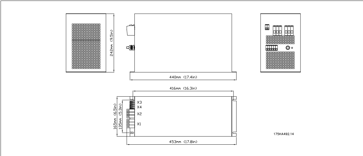
Illustration 3.1: Frame size B
