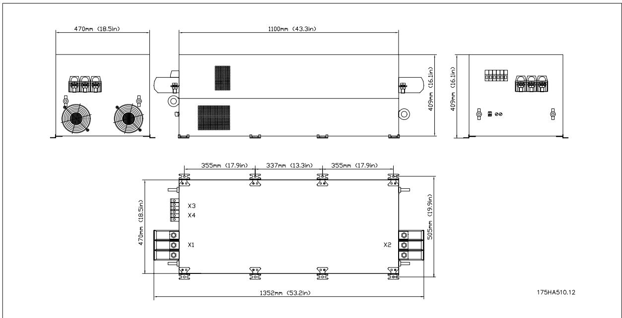
Illustration 3.7: Frame size H
