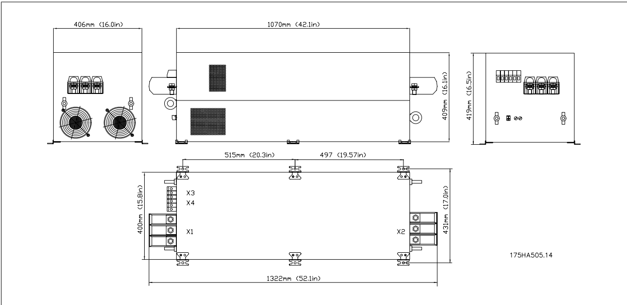
Illustration 3.6: Frame size G
