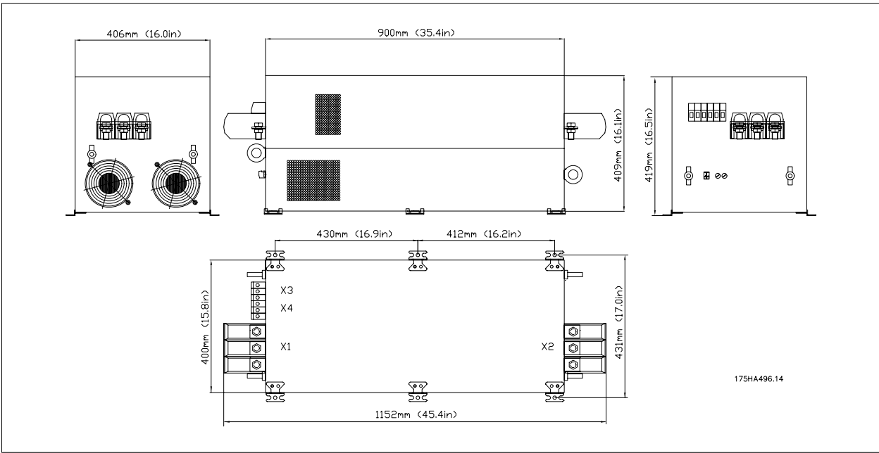
Illustration 3.5: Frame size F
