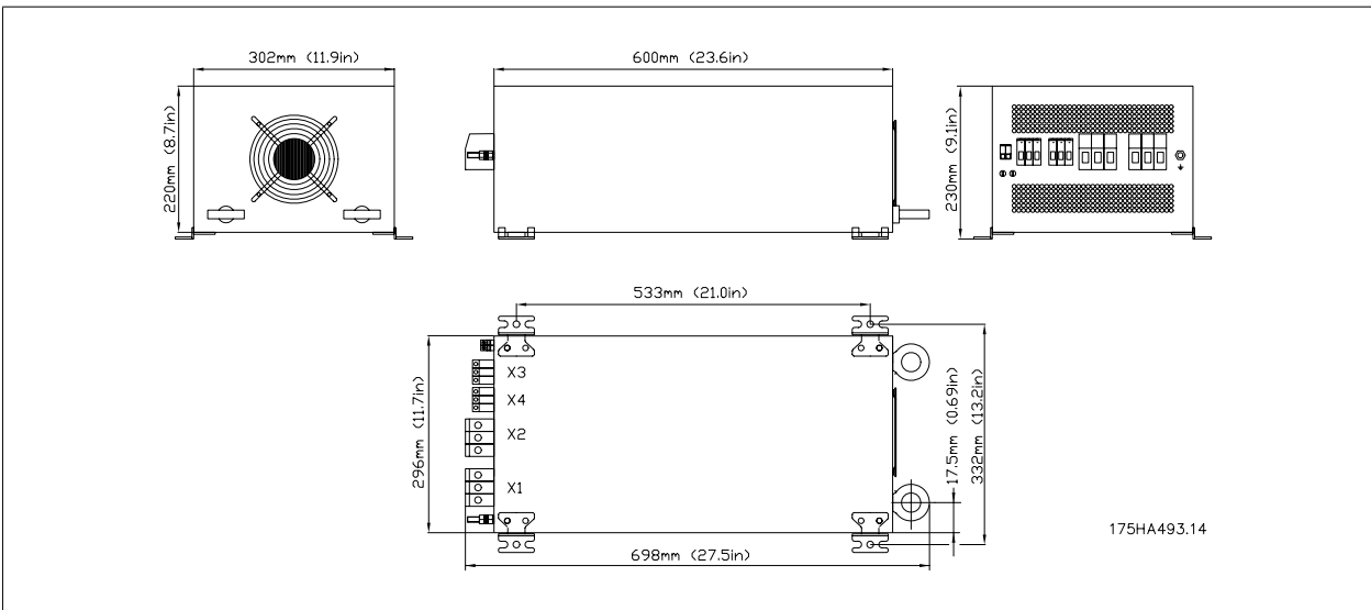
Illustration 3.2: Frame size C
