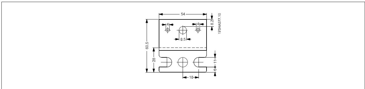
Illustration 3.8: Detailed drawing of mounting feet.
