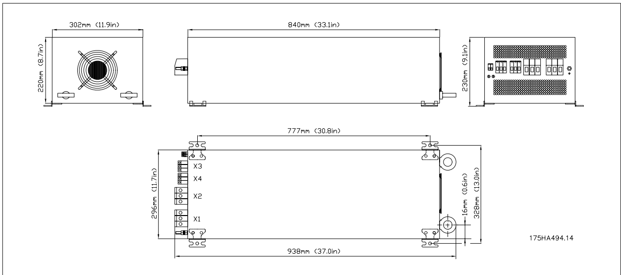
Illustration 3.3: Frame size D
