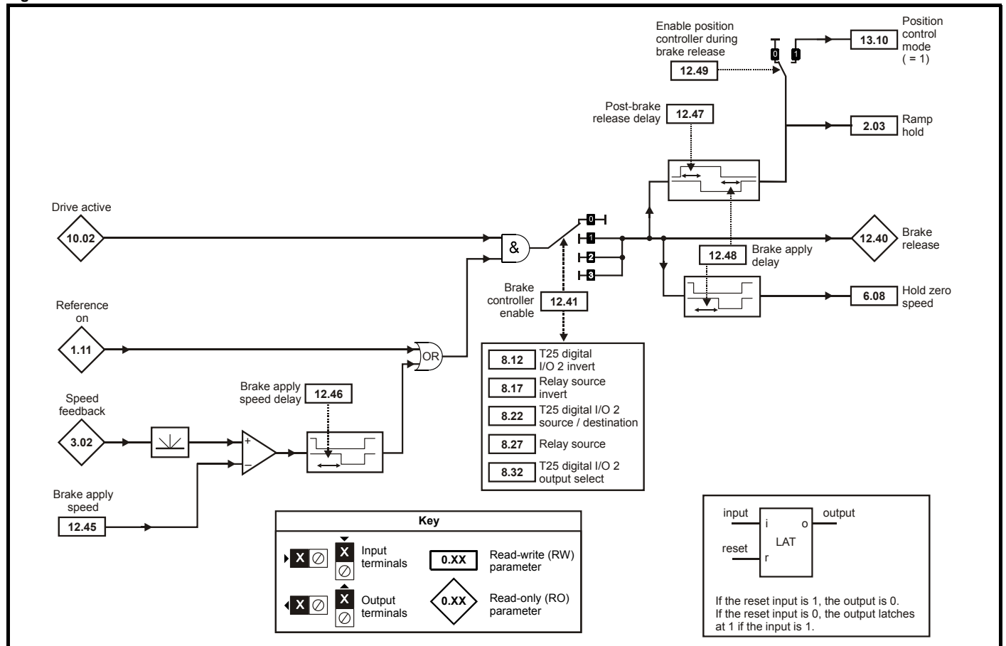
Figure 5-13 Brake function
