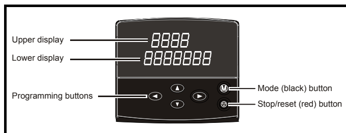
Figure 2-1 Digitax ST Keypad
