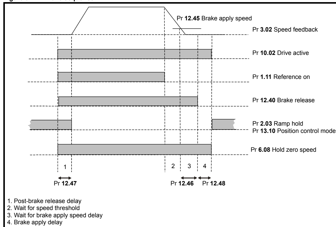
Figure 5-14 Brake sequence
