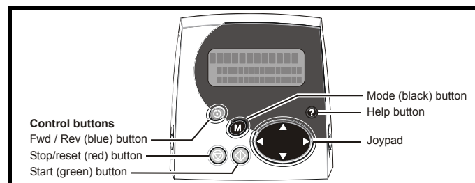
Figure 2-2 SM-Keypad Plus (remote mount only)
