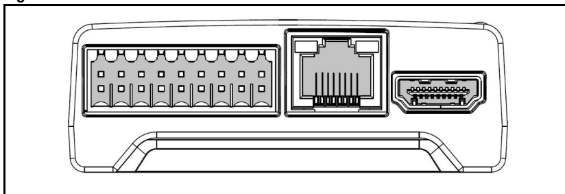
Figure 4-3 Encoder interface
