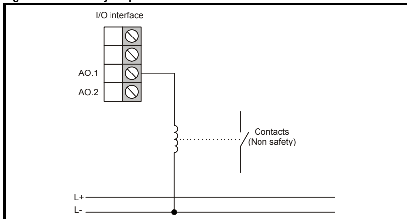
Figure 3-17 Auxiliary output circuit
