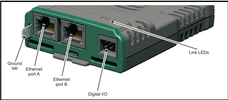
Figure 4-2 MCi210 Connections
