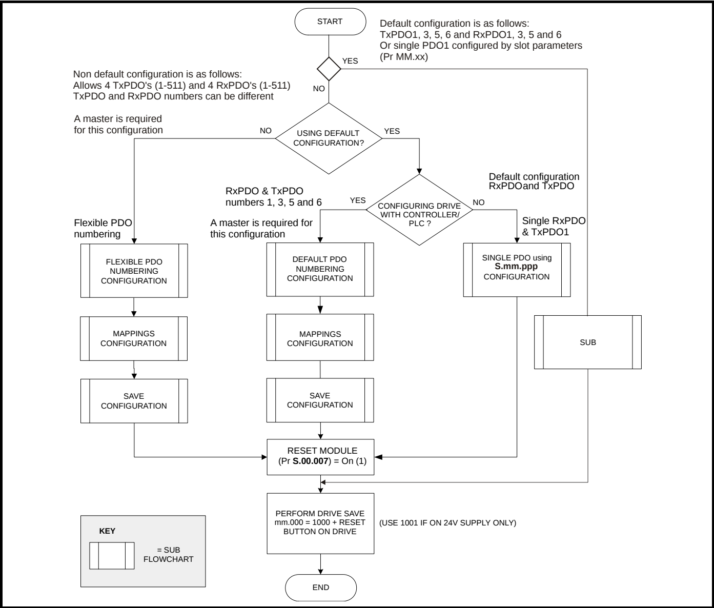
Figure 5-3 Configuration options flowchart
