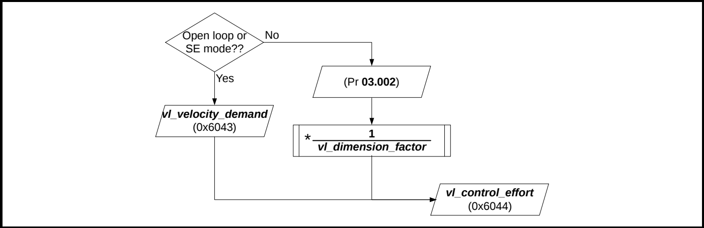
Figure 11-6 vl_control_effort
