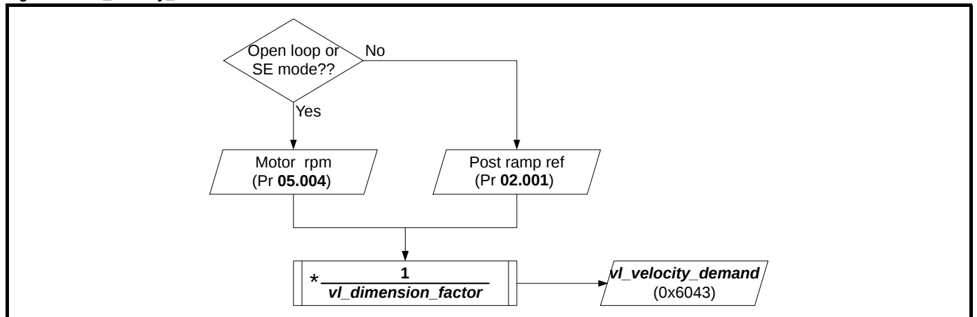
Figure 11-5 vl_velocity_demand
