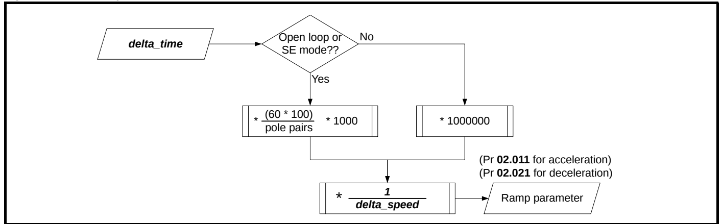
Figure 11-7 vl_velocity_acceleration
