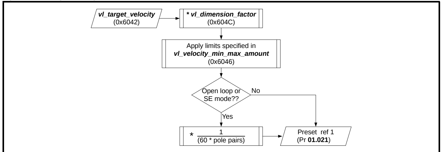
Figure 11-4 vl_target_velocity
