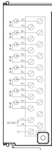
SM3A18C
