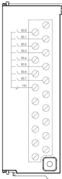
SM3DI8
