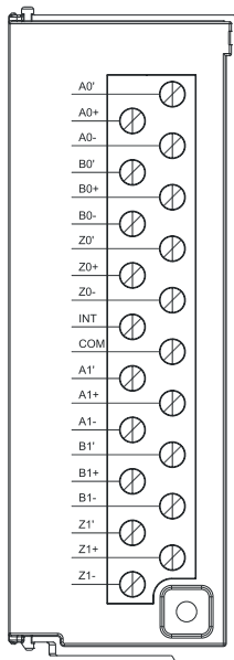
HSC-02
