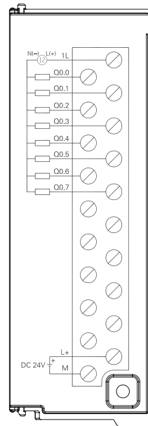
SM3DQ8R
