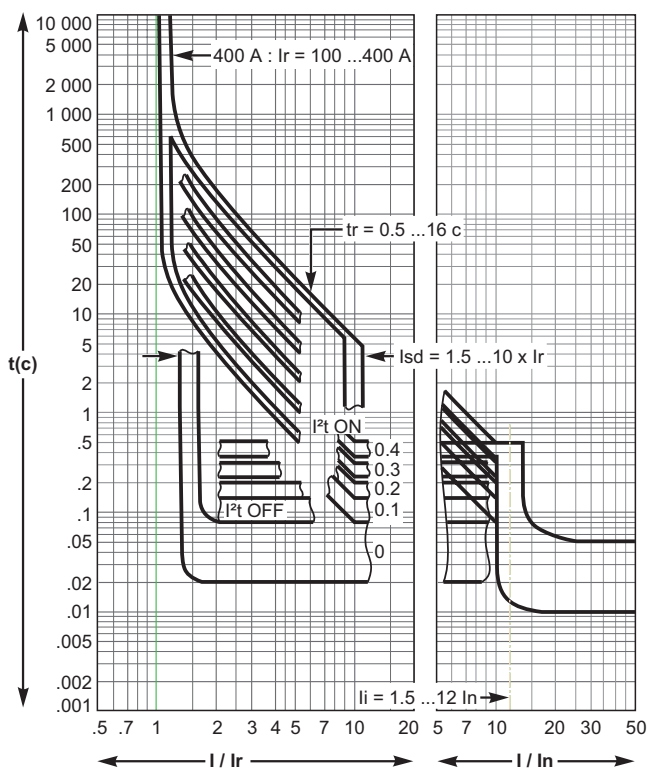
SystemeLogic 5.3E 400
