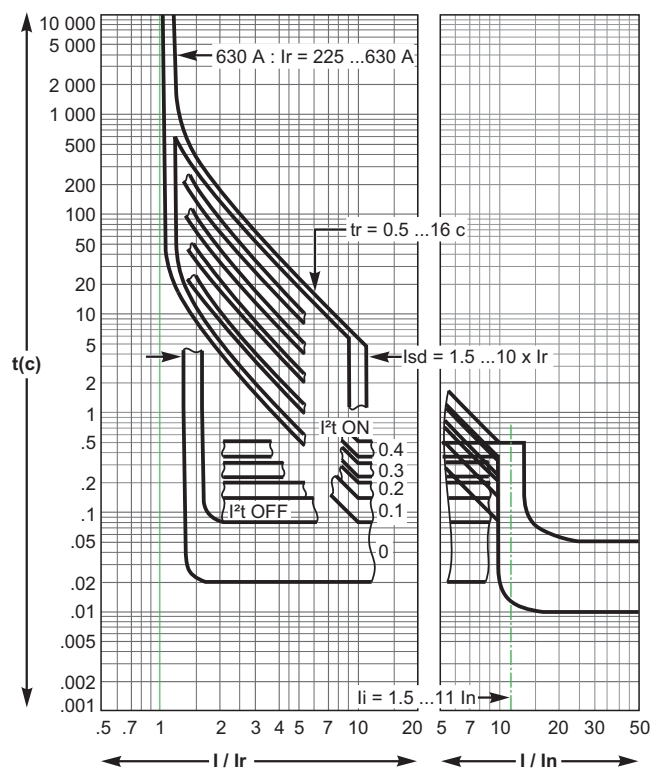
SystemeLogic 5.3E 630
