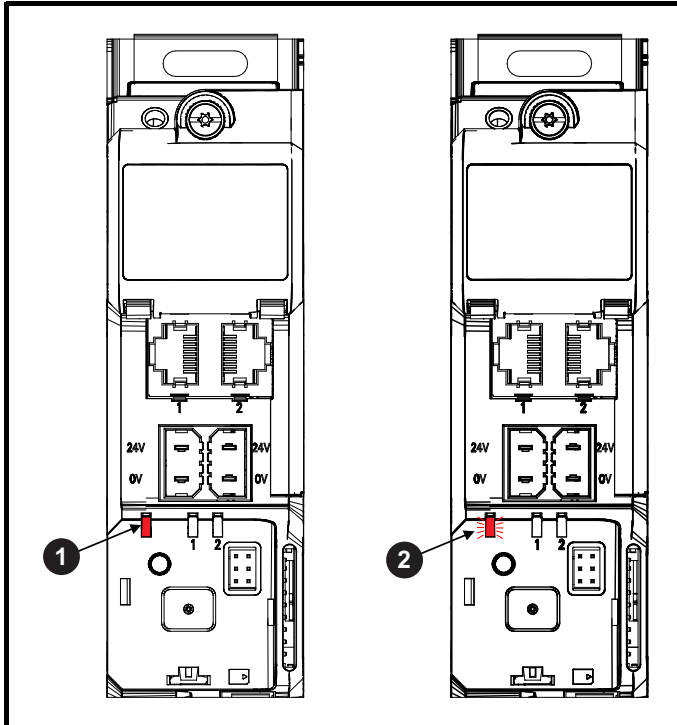
Figure 12-3 Location of the status LED
