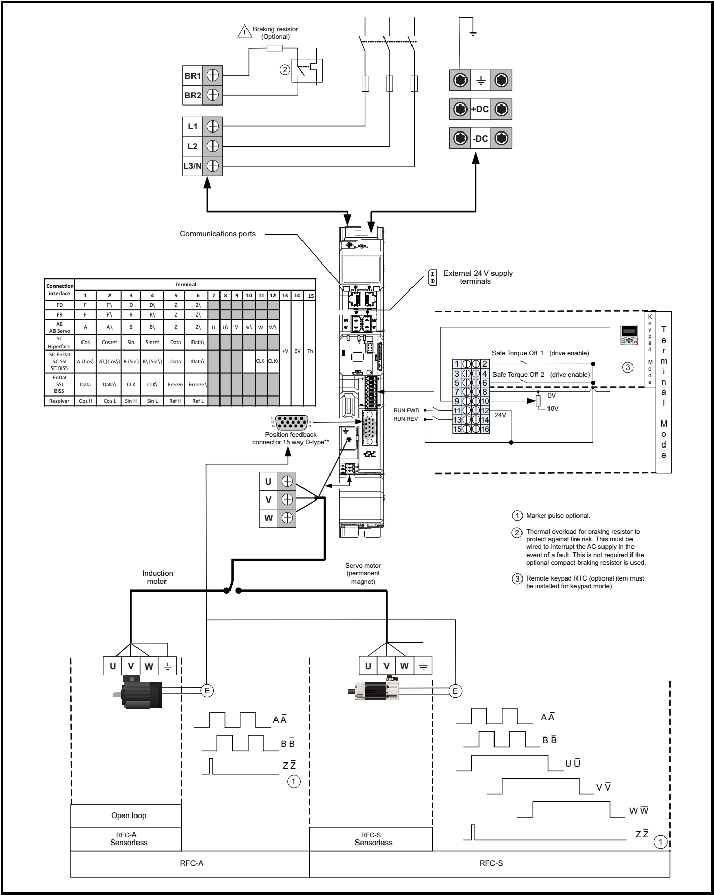
Figure 7-1 Minimum connections to get the motor running in any operating mode for Digitax HD M75X (all frame sizes)
