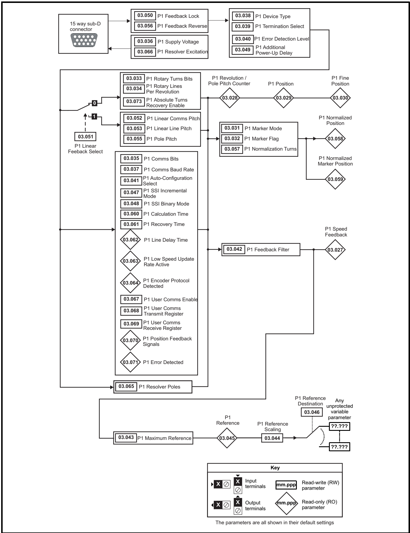
Figure 11-5 P1 Interface
