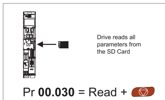
Figure 9-2 Basic SD Card operation
