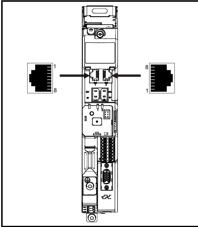
Figure 5-9 Location of the comms connectors
