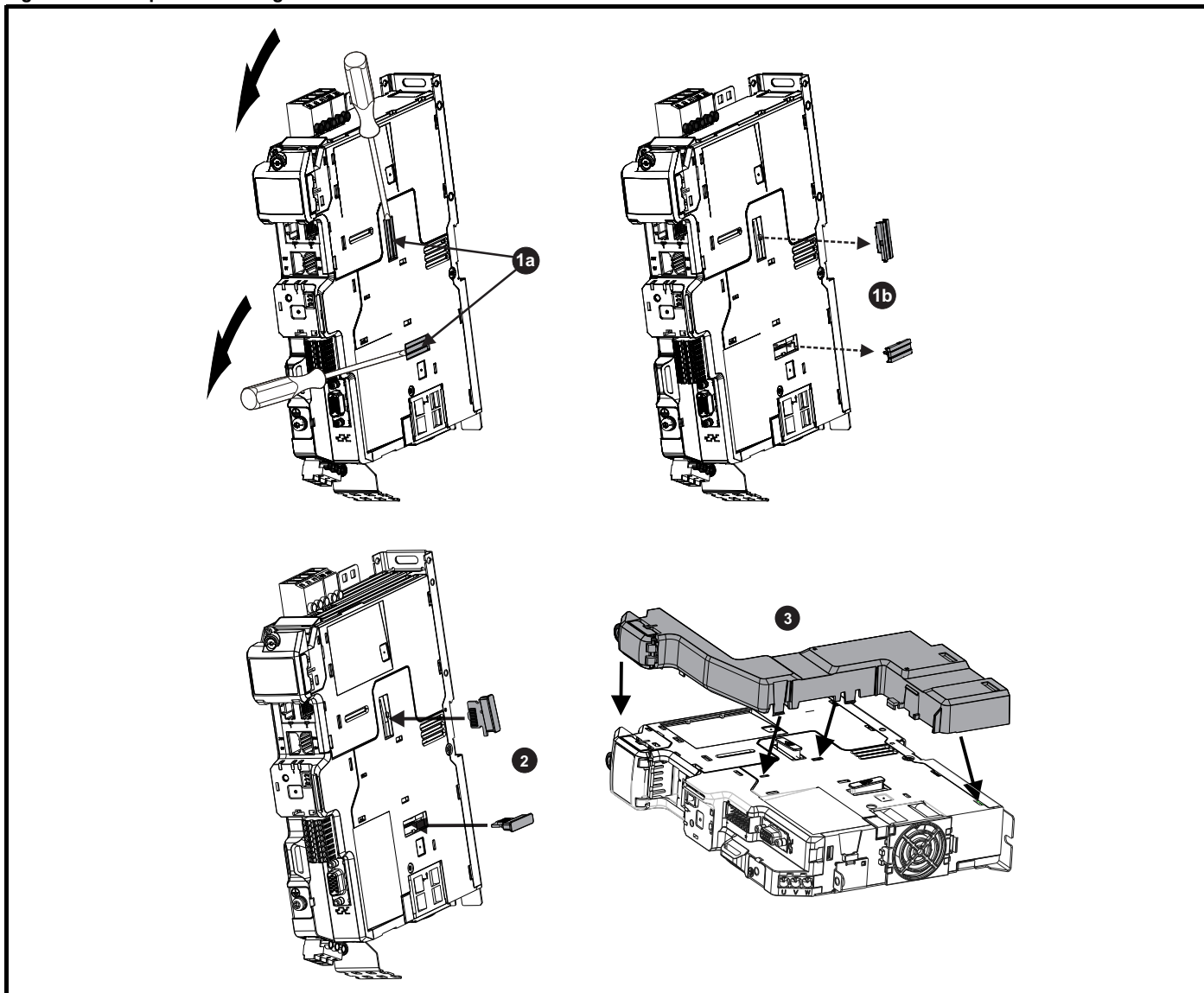
Figure 3-1 SI-Option mounting kit Installation
