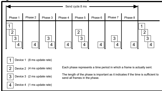
Figure 9-5 Profinet transmission cycle
