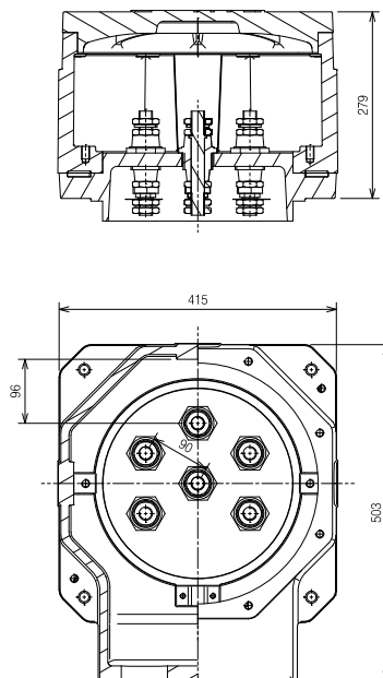
Frame size 355
