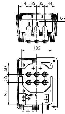
Frame size 160 - 200
