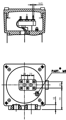
Frame size 90 - 132
