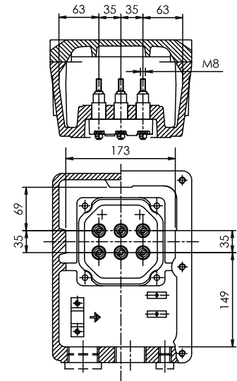
Frame size 400 - 450
