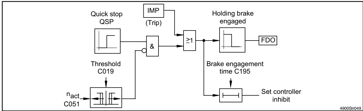
FIG 7-22 Block diagram 'Engage brake'
